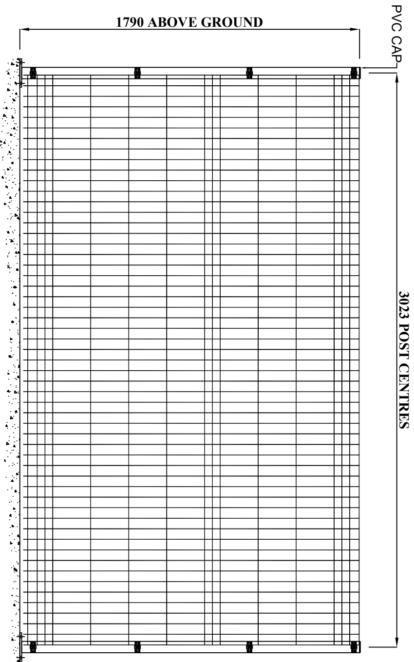
NK IBEX ECO - TYPICAL ELEVATION - 1.80 HIGH BASEPLATED FENCE
