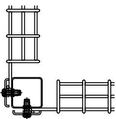
CONFIGURATION @ INTERMEDIATE POST
