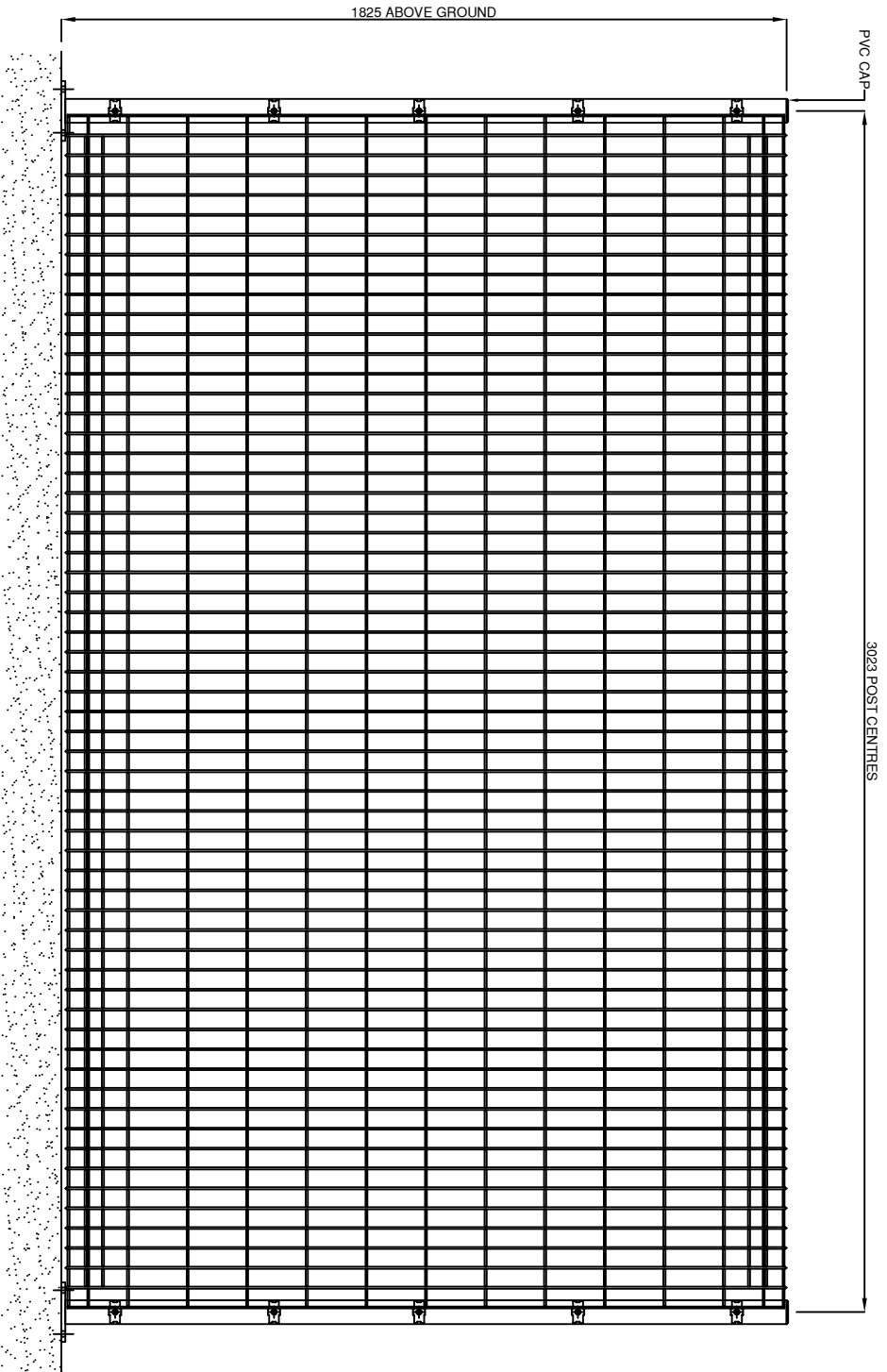
NK IBEX SAFETOP - TYPICAL ELEVATION ON STD FENCE PANEL - 1.80 HIGH BASEPLATED FENCE
