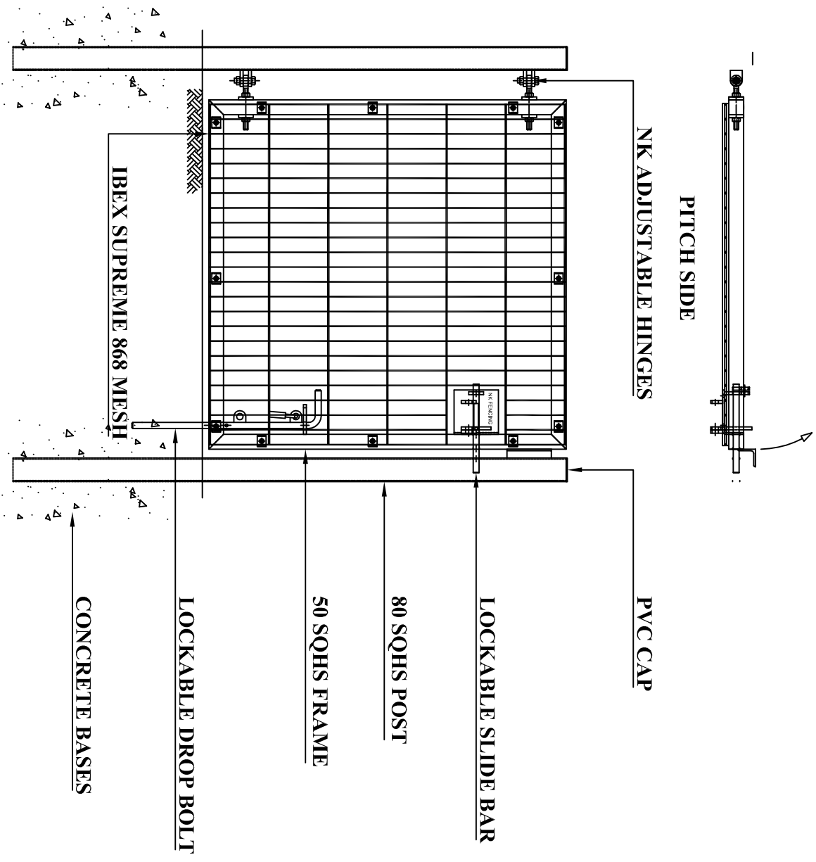
NK SPORTS PITCH SURROUND S/L GATE - TYPICAL ELEVATION
